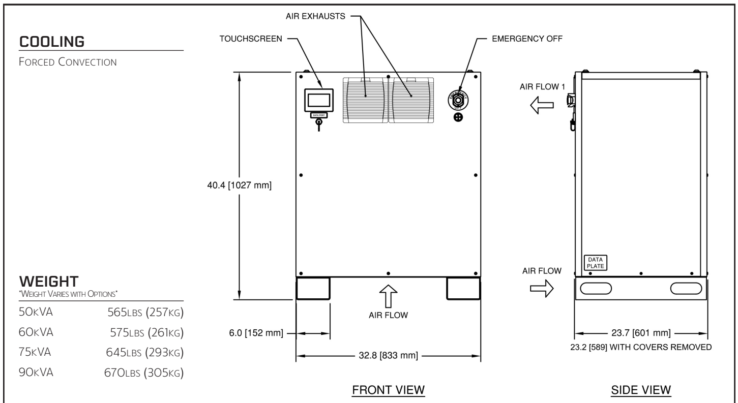
FIGURE 1 – ShorePOWER Ultra HF 50-90kVA
