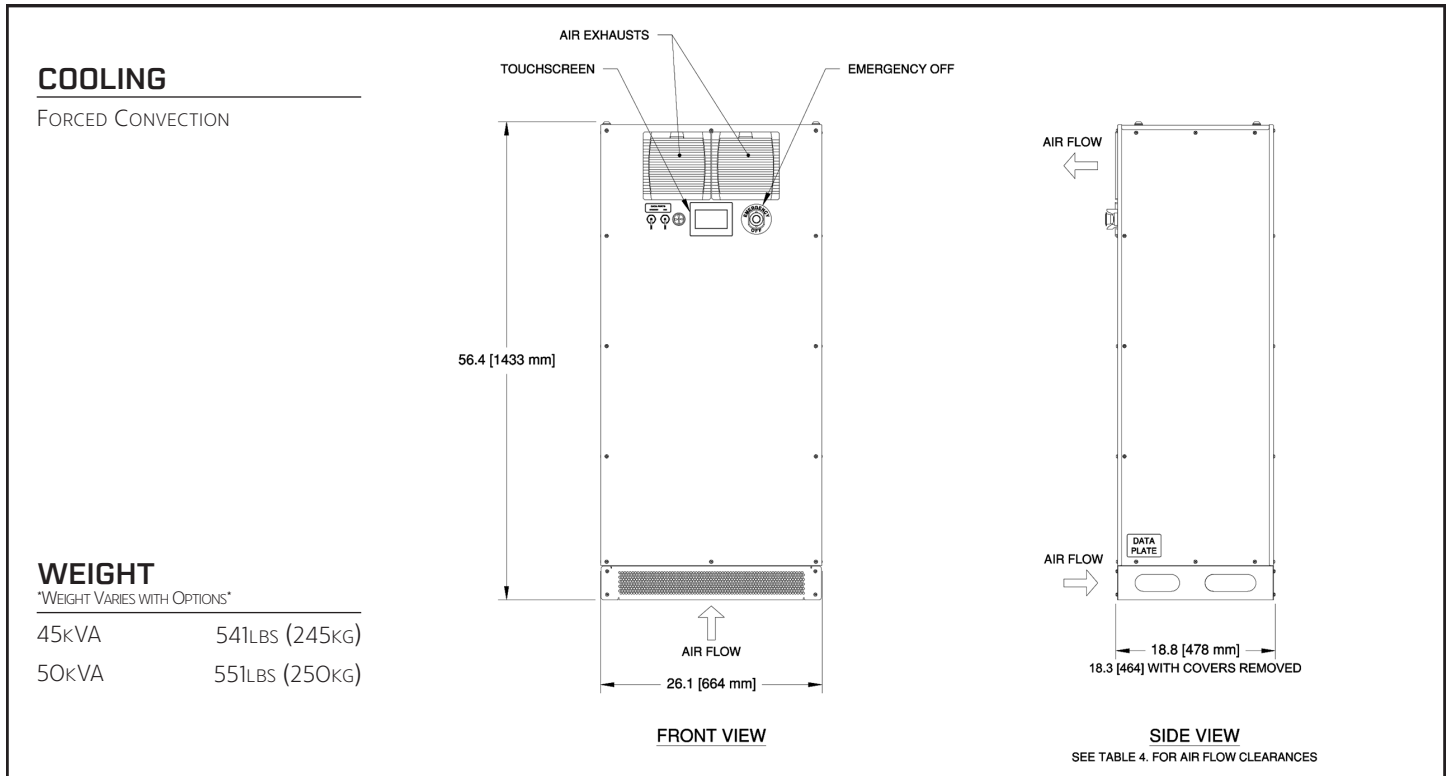
FIGURE 1 – SHORPOWER SHF 45-50kVA – F-CABINET
